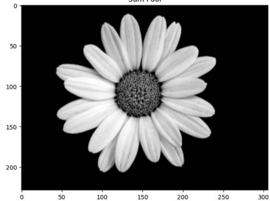
Sum Pool
