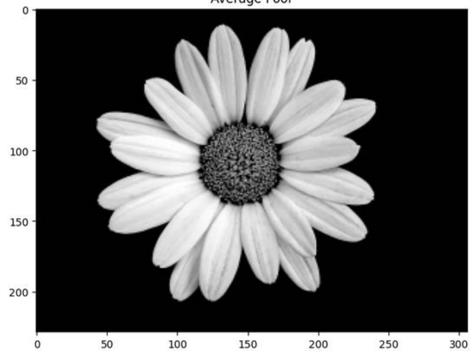
Average Pool
